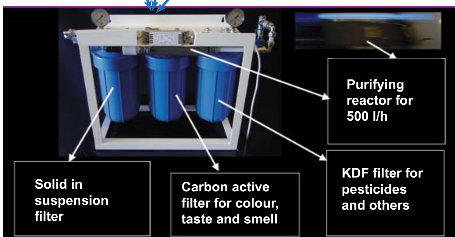
DETAIL OF THE SERVICE PURIFIER. 500 l/h.
