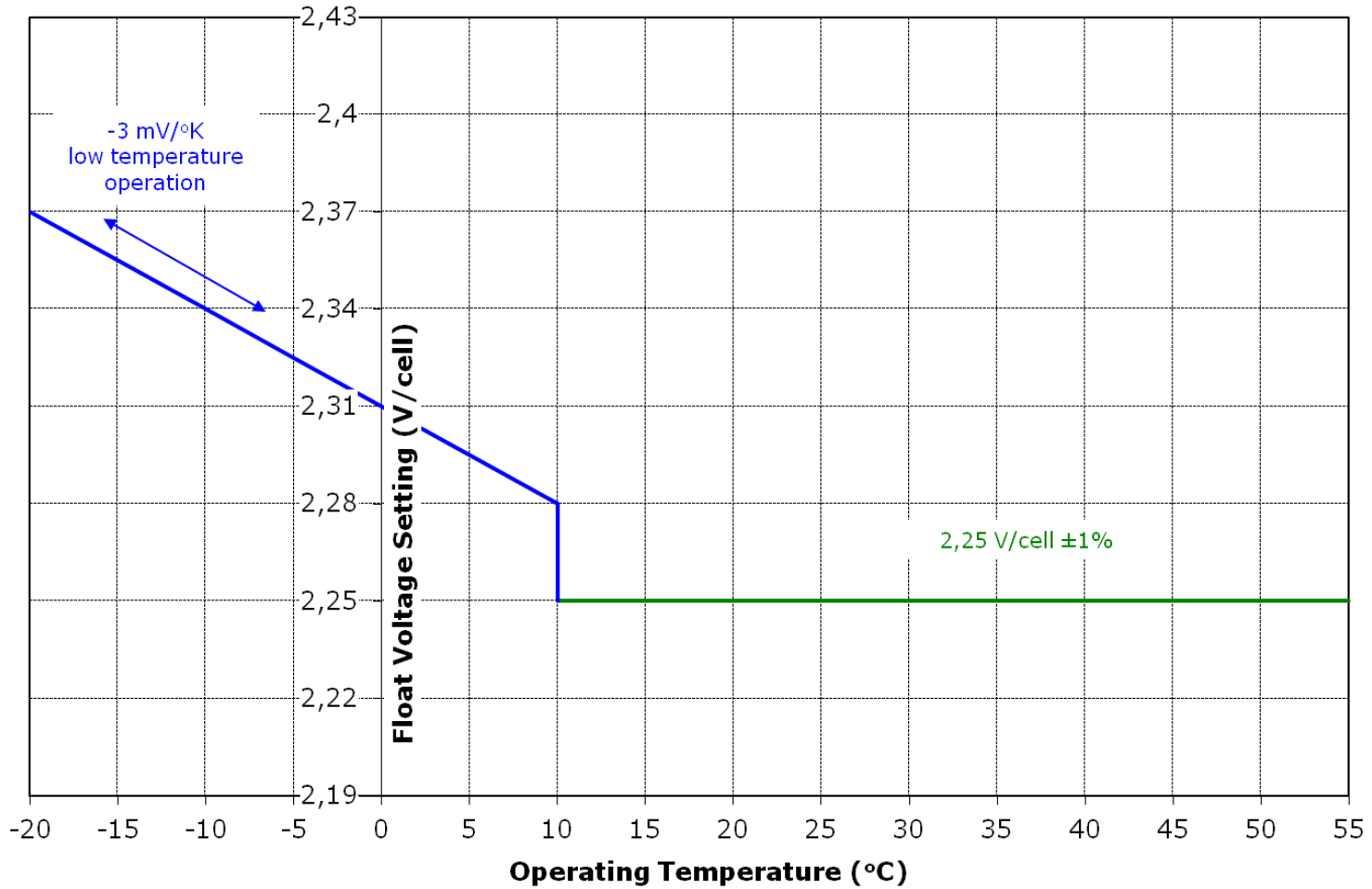
OPzV - Float Voltage Setting Vs Operating Temperature
