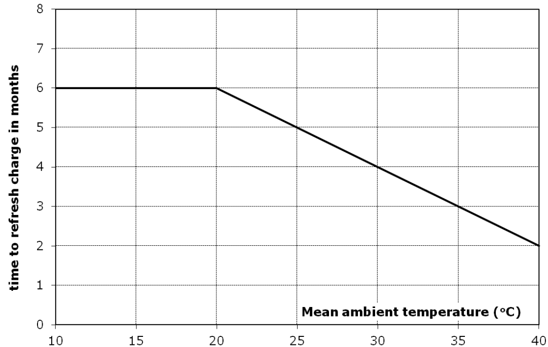
OPzV - Recommended time to refresh charge during prolonged storage
